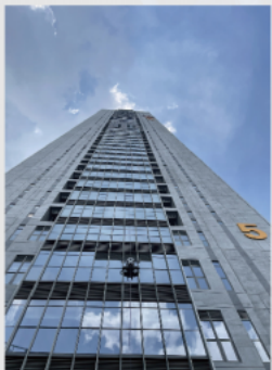
Super high-rise composite curtain wall
